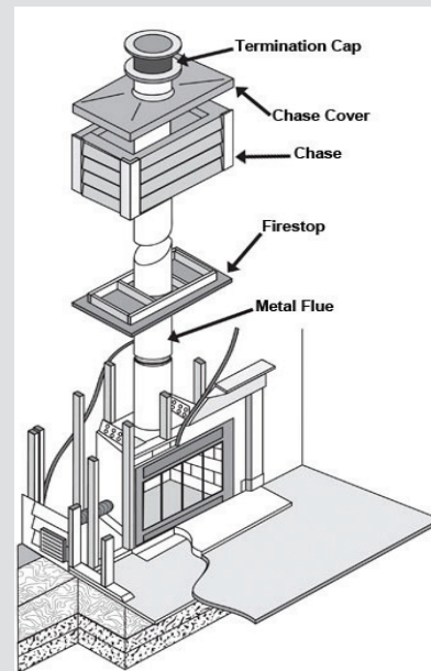
Zero Clearance fireplace
